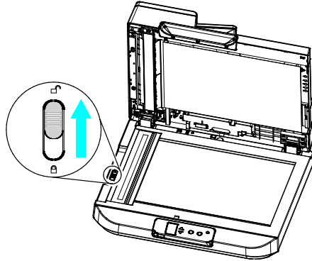
Figure 2-1 Unlocking the Scanner
