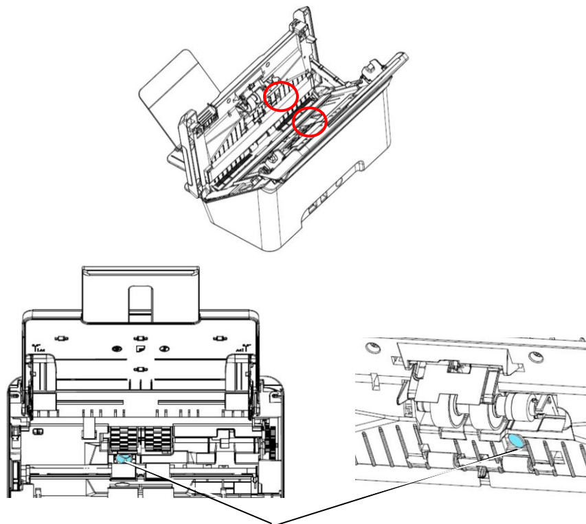
Ultrasonic sensors
